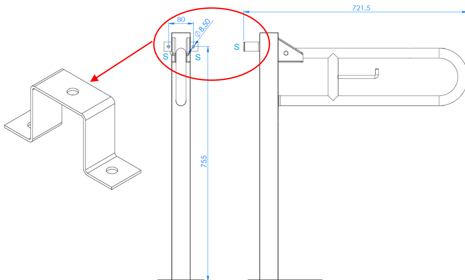
Wall fixing
